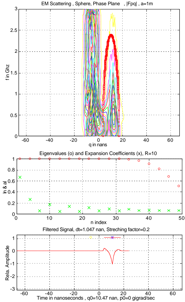
Figure 4. Electromagnetic scattering from sphere. Filtered signal with N = 50 degrees of freedom. Filtered is displaced by \pi nans. Radius a = 1\text{ m} .
